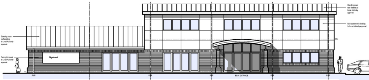
FRONT ELEVATION
